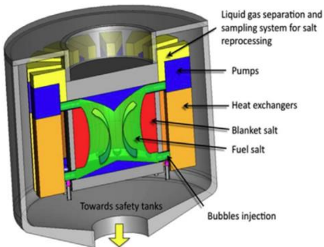
Figure 2.1. Concept design with basic components shown of the TMSR (Serp, et al., 2014)
